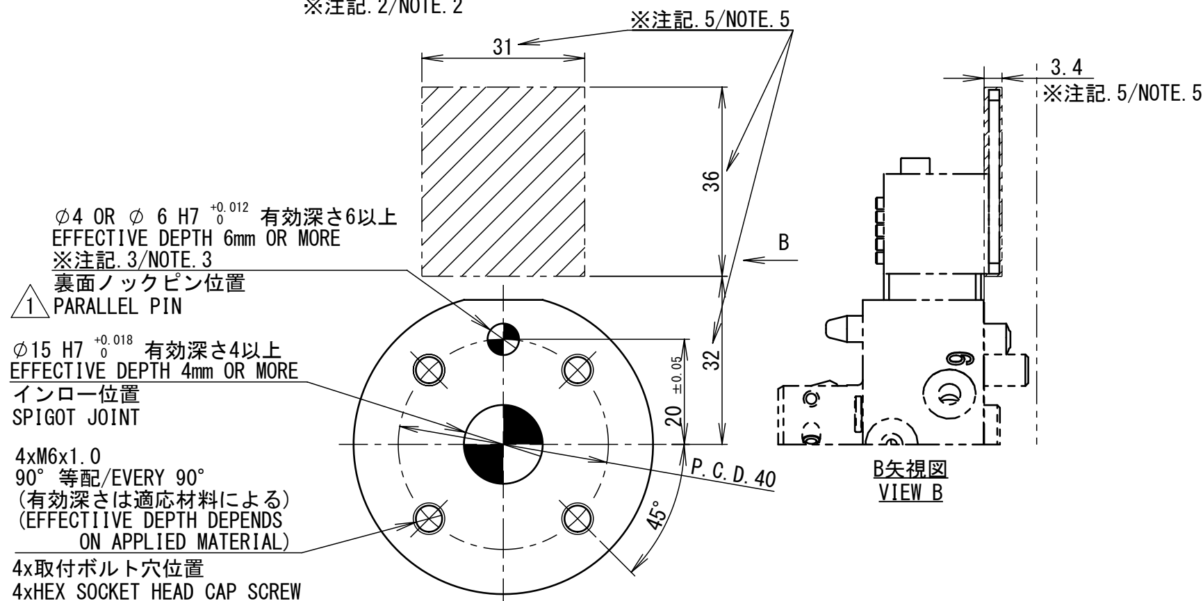
取合寸法図 (A矢視図) CONNECTING DIMENSION VIEW (VIEW A)
