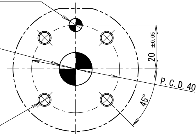
取合寸法図 (A矢視図) CONNECTING DIMENSION VIEW (VIEW A)
