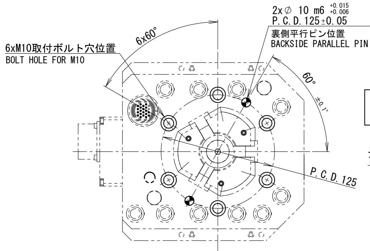
矢視図A: 取合い寸法図 VIEW A: CONNECTING DIMENSION VIEW
