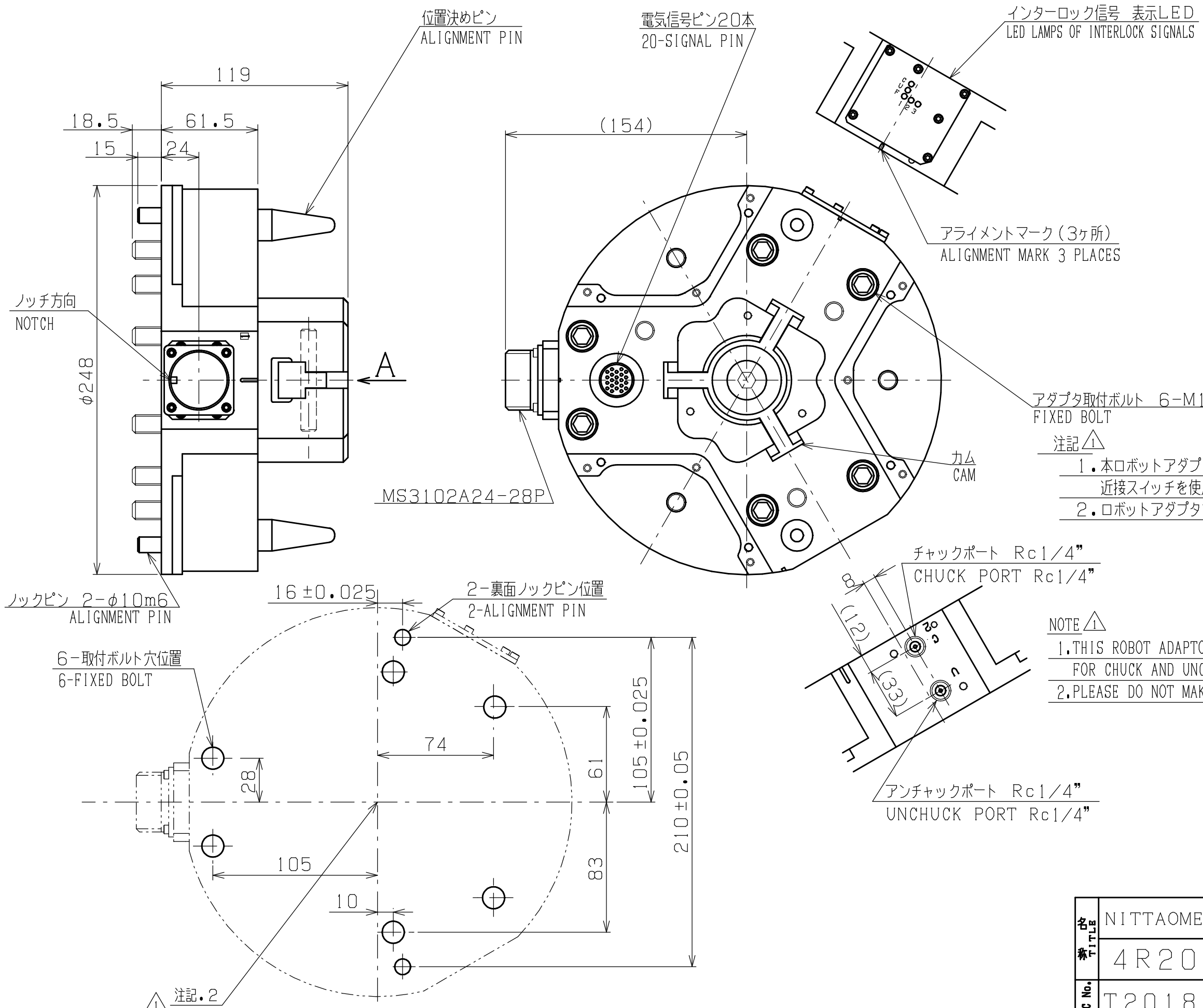
取合寸法図 (A矢視) CONNECTING DIMENSION VIEW (VIEW A)
