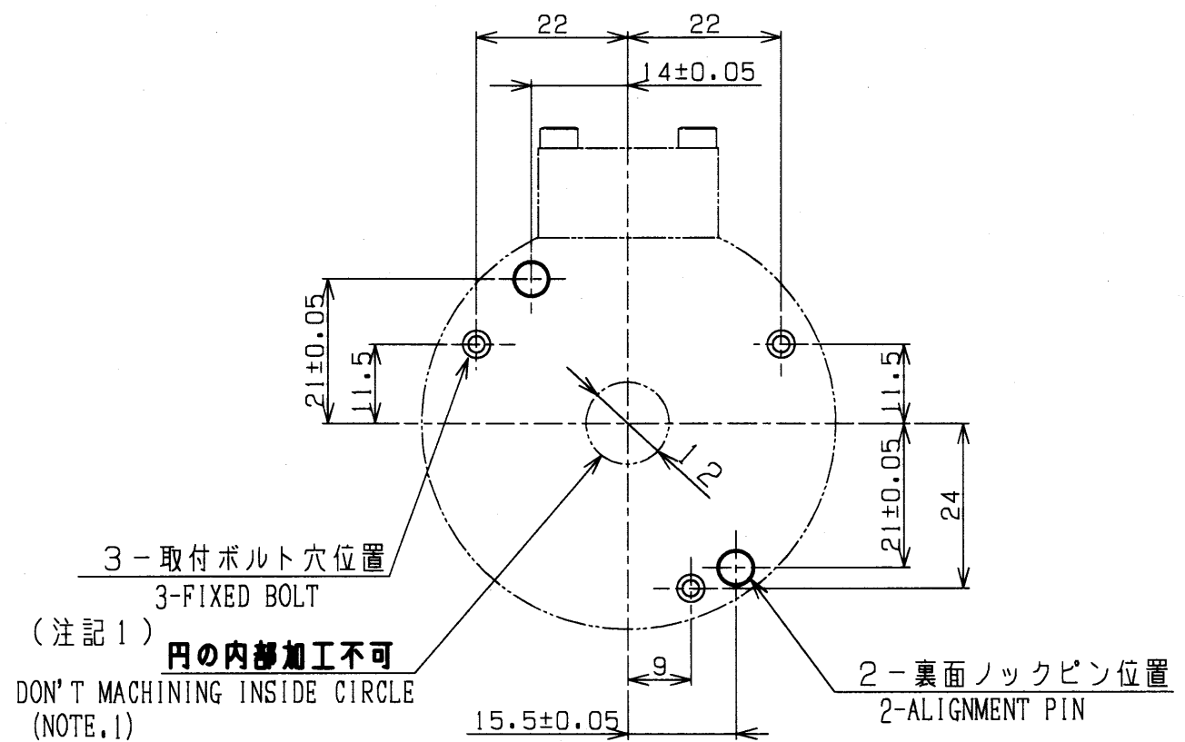
取合寸法図 (A 矢視図) CONNECTING DIMENSION VIEW (VIEW A)
